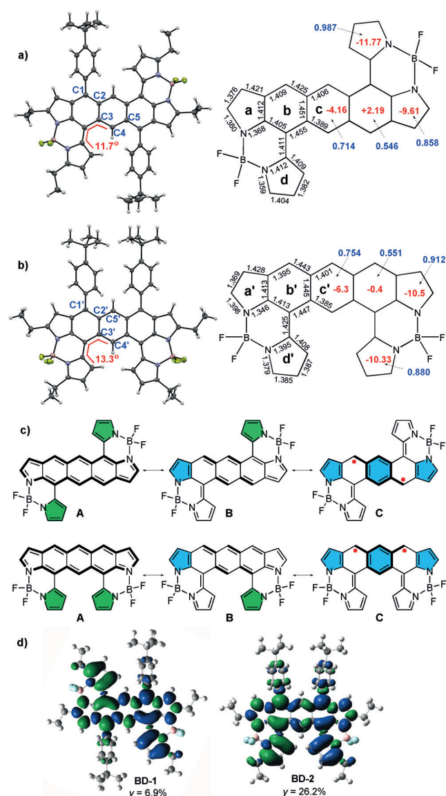
Figure 2. ORTEP representations and mean bond lengths (Å) for the crystal structures of a) BD-1 and b) BD-2 . The red and blue numbers are the calculated NICS(1) zz and HOMA values of the selected rings, respectively. c) Different resonance forms for BD-1 and BD-2 . The blue and green surfaces represent \alpha and \beta spin densities, respectively. d) Calculated (UB3LYP/6-31G*) spin density distributions of BD-1 and BD-2 in the singlet diradical form.
